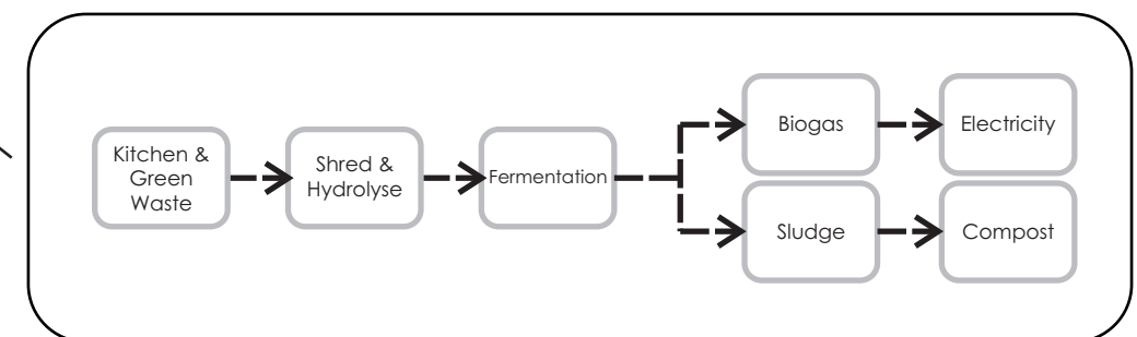
Anaerobic Digestion Process
