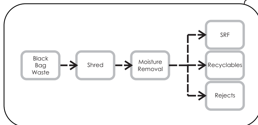
Mechanical Biological Treatment Process
