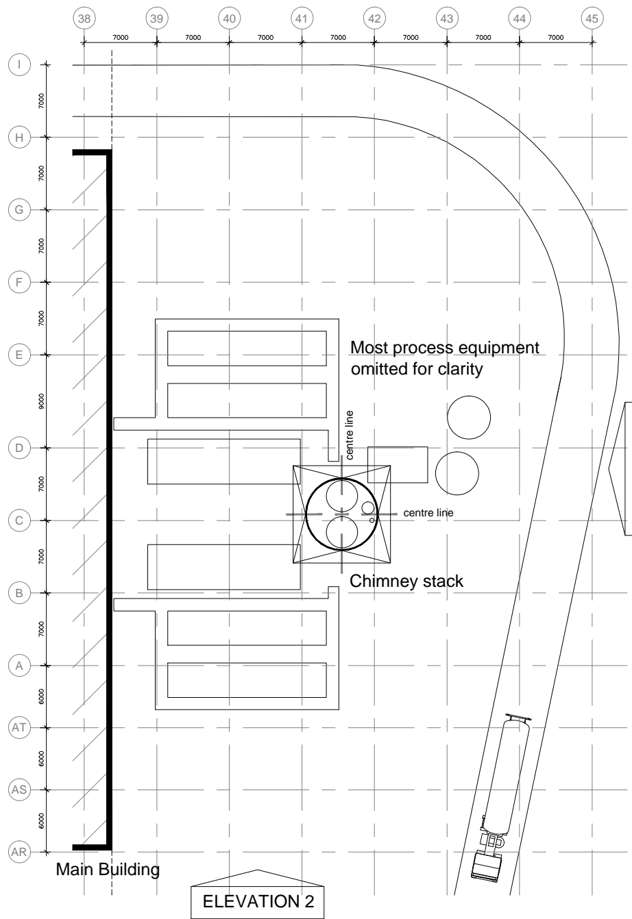
PLAN
