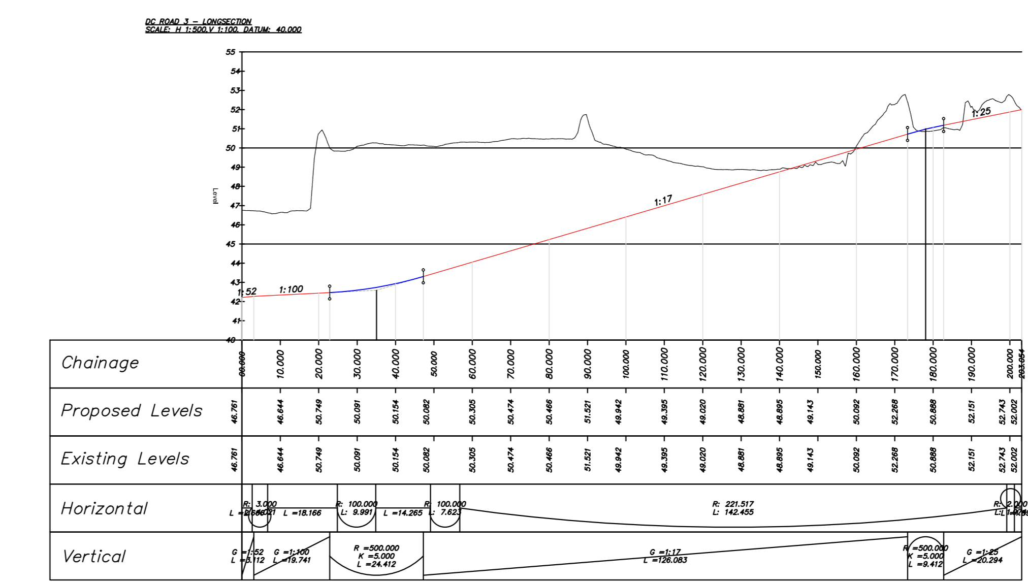
Road 3 Longitudinal Section Scale 1:1000
