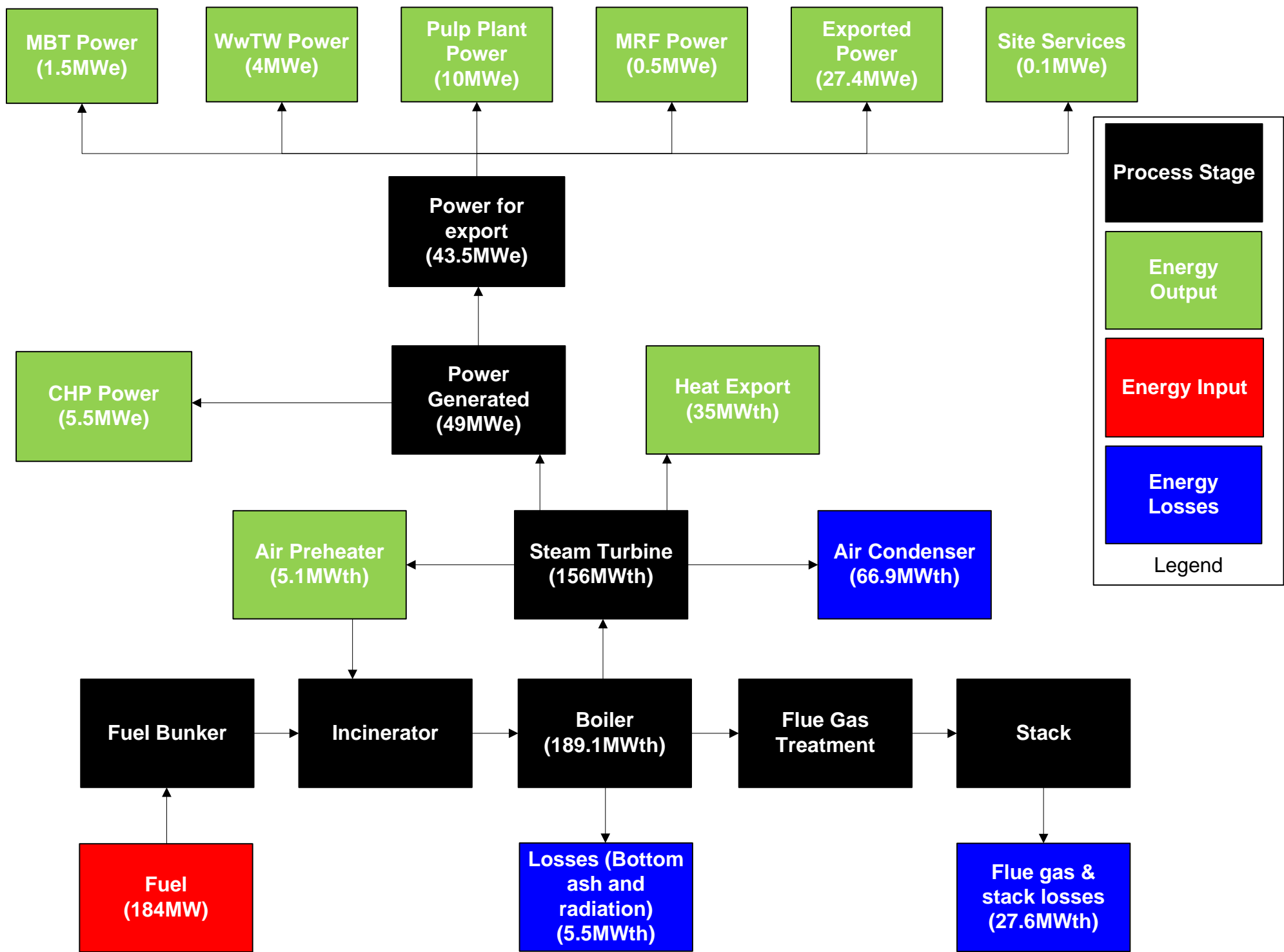
CHP Energy Flow Diagram
