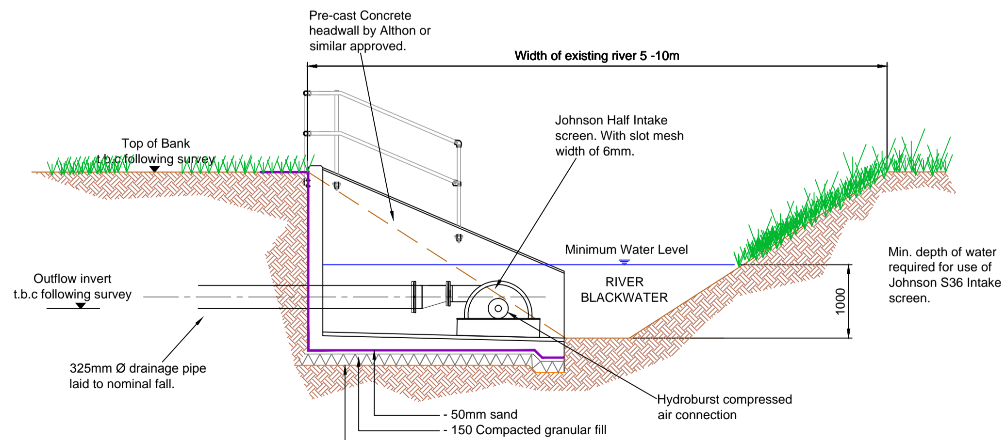
SECTION THROUGH BLACKWATER RIVER ABSTRACTION - FOR SHALLOW WATER (1:50)
