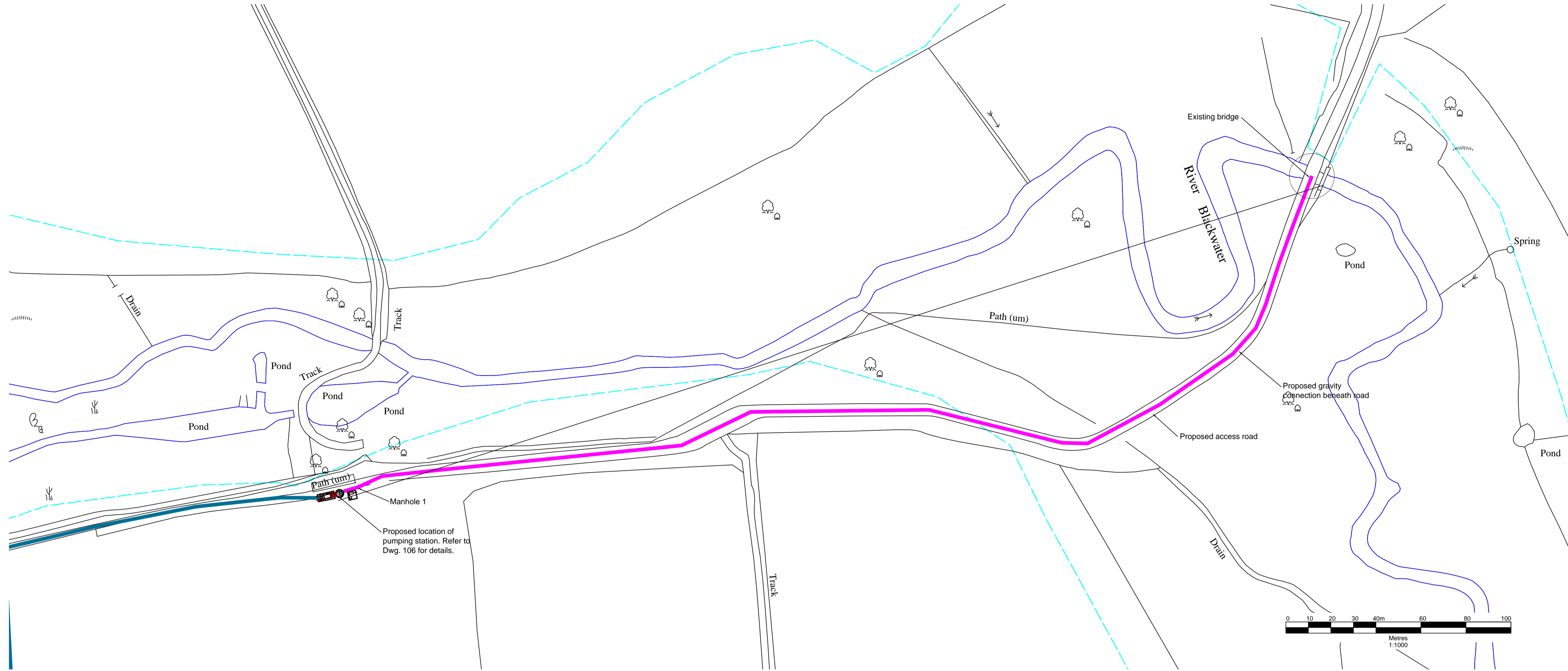
PLAN ON PROPOSED RIVER BLACKWATER ABSTRACTION (1:1000)
