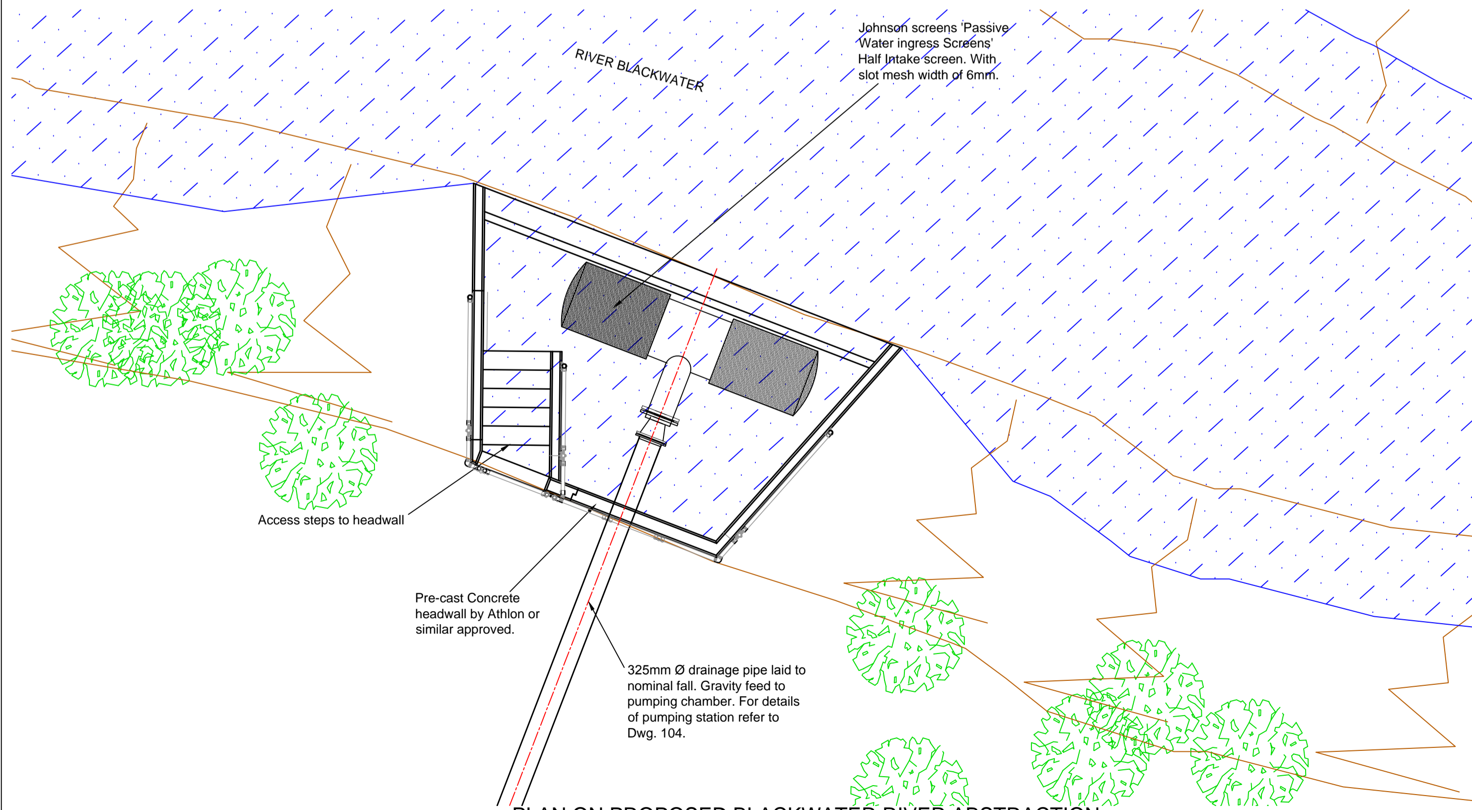
PLAN ON PROPOSED BLACKWATER RIVER ABSTRACTION (1:50)
